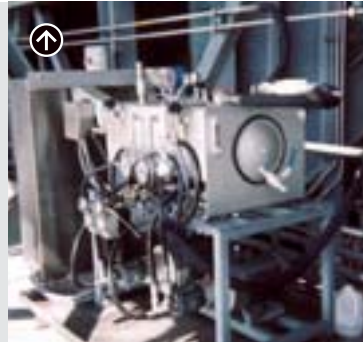
High Pressure Hydraulic Power Unit Delta II Rocket Launch Tower Hydraulic System
